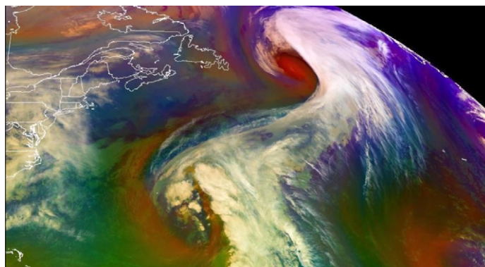
This GOES-16 air mass RGB imagery shows a pair of mid-latitude cyclones in the North Atlantic on Jan. 23, 2020. This type of imagery combines water vapor and infrared imagery and is used to monitor the evolution of cyclones and jet streaks. Credit: NOAA/CIRA
