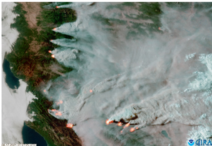
GOES-17 imagery of numerous fires burning in California on Aug. 17, 2021, combines GeoColor imagery with the fire temperature data product to highlight both the fires' hotspots and smoke plumes. Credit: NOAA/CIRA
